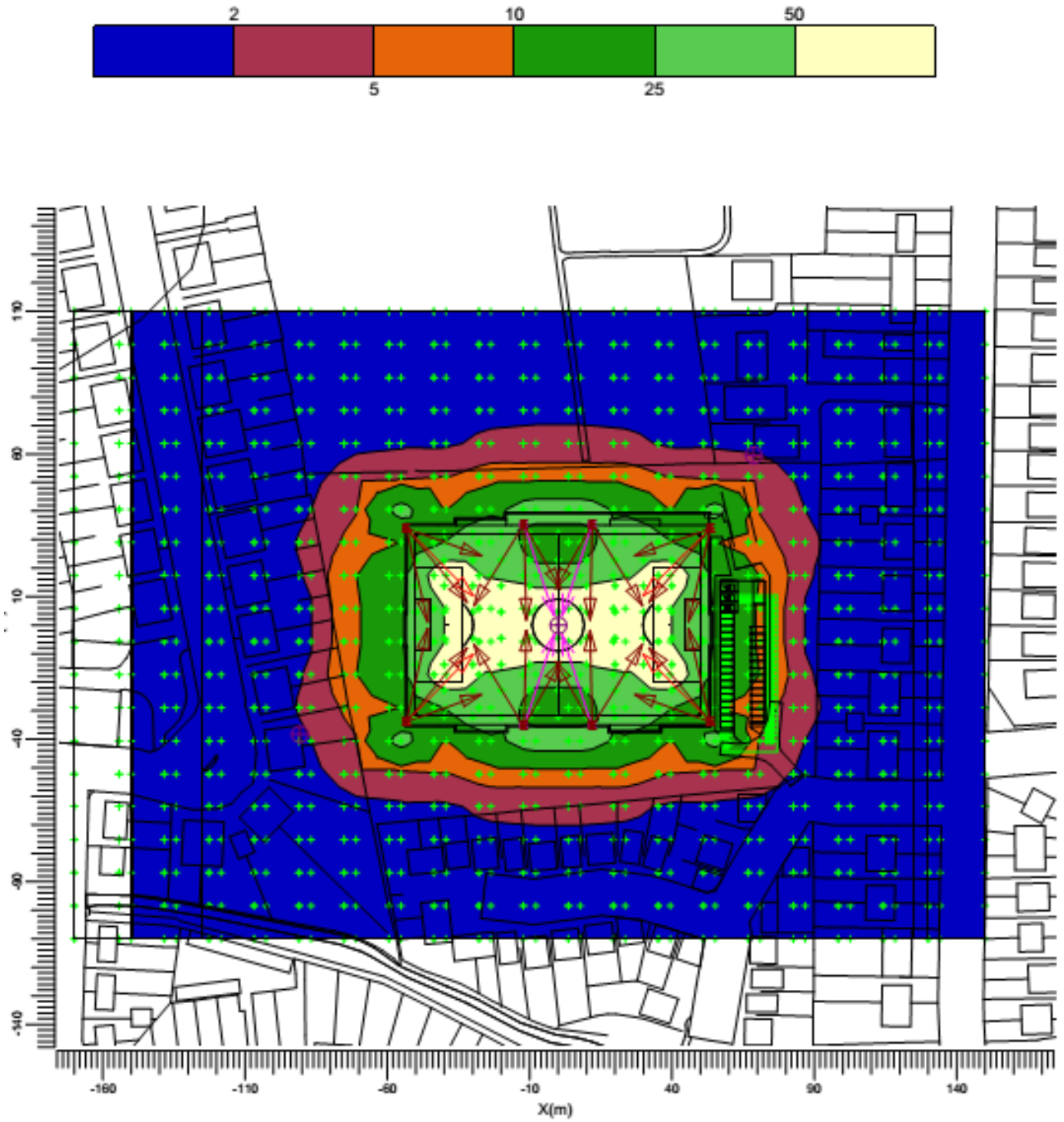
A - 200 Lux Spillage Diagram
