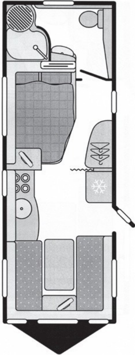
Model 625
