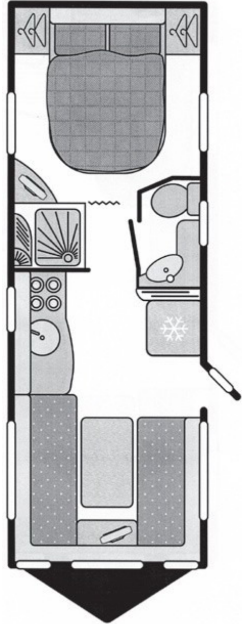
Model 645
